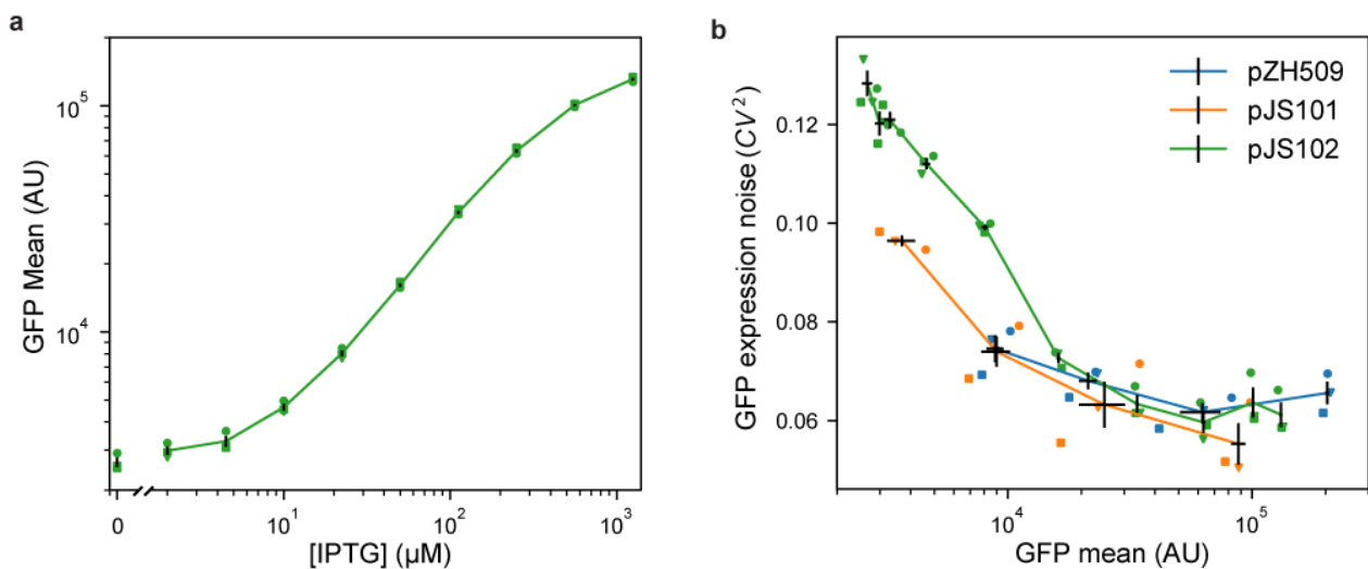
Figure 2: Characterizing mean expression levels and noise for different gene expression systems. Cultures of E. coli MG1655 harboring pJS102 (LacI regulation, p15a origin, green), pZH509 (TetR regulation, p15a origin, blue) or pJS101 (TetR regulation, pSC101 origin, orange) were grown at 30 °C in rich media with induction by IPTG (0, 2, 4.5, 10, 22.4, 50, 111.8, 250, 559 and 1250 \mu\text{M} ) or ATc (1, 5, 25 and 125 nM). Mean single-cell GFP fluorescence and GFP expression noise was estimated using flow cytometry. Data from 3 independent replicates are indicated with different shapes. Black lines indicate the mean GFP expression and expression noise plus or minus 1 standard error of the mean from the 3 replicates. (a) Mean GFP expression for pJS102 at different IPTG concentrations shows tunable and reproducible induction over an \sim 50 -fold dynamic range. Expression at zero IPTG is plotted separately to fit on logarithmic scale. (b) GFP expression noise as a function of mean for pZH509, pJS101 and pJS102. For all samples, GFP mean increases monotonically with inducer concentration. Note that the full range of induction is not shown here for pZH509 and pJS101 as even 1 nM ATc induces expression. GFP expression noise is low in all conditions for all strains.
